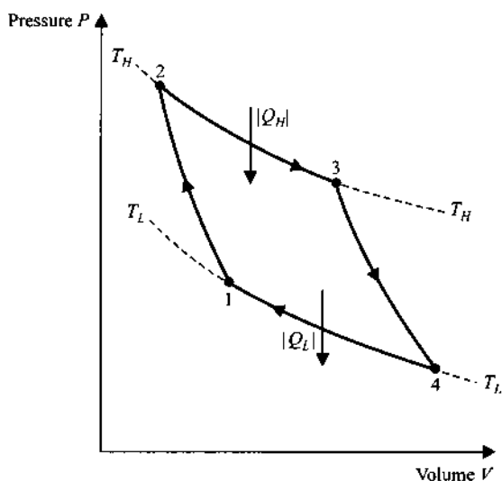
FIGURE 7-1 Carnot cycle of a real gas.
