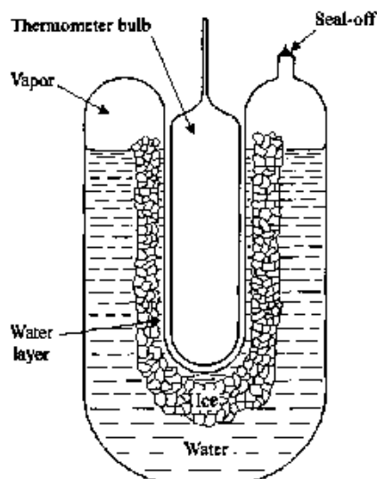
FIGURE 1-5 Triple-point cell.
