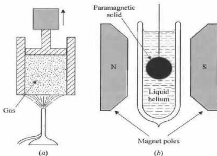
FIGURE 4-4 Nonadiabatic processes.
